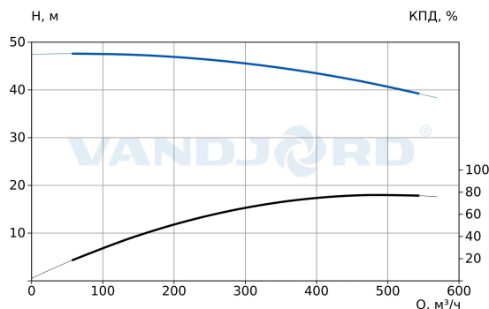
73121113 TPV 200-420-75/4 Q-A-B-E
