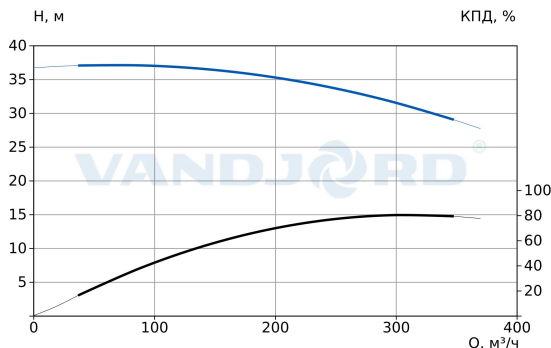
73119107 TPV 150-320-37/4 Q-A-B-E
