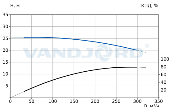
73119105 TPV 150-220-22/4 Q-A-B-E
