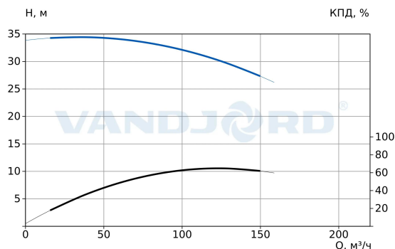
73117130 TPV 100-300-18.5/4 Q-A-B-E
