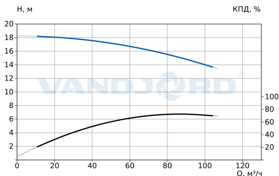
73117126 TPV 100-150-5.5/4 Q-A-B-E
