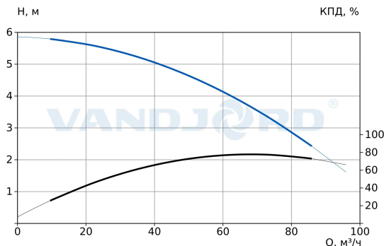
73117120 TPV 100-50-1.1/4 Q-A-B-E
