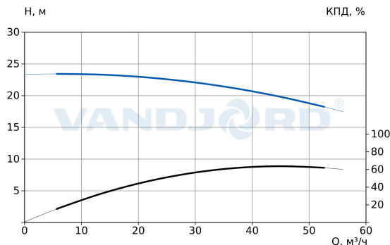
73115118 TPV 65-200-4/4 Q-A-B-E
