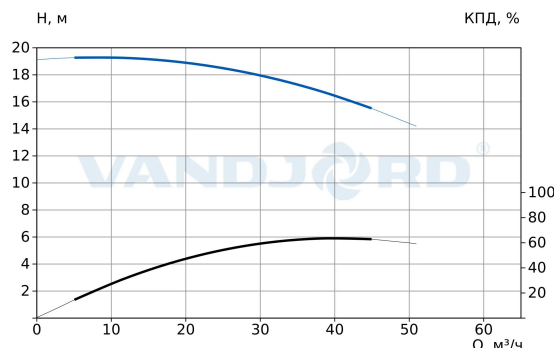
73115117 TPV 65-160-3/4 Q-A-B-E
