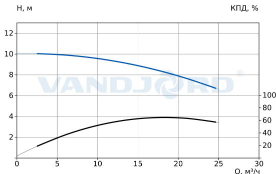
73114113 TPV 50-80-0.75/4 Q-A-B-E
