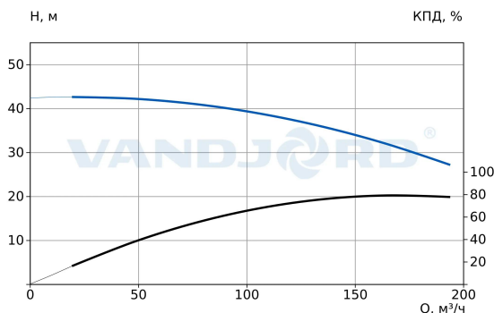
73117107 TPV 100-320-22/2 Q-A-B-E
