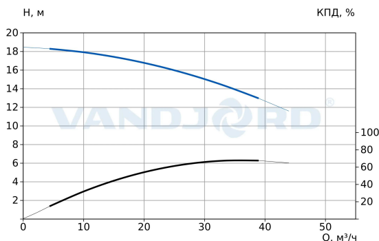
73115101 TPV 65-150-2.2/2 Q-A-B-E
