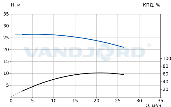
73113105 TPV 40-230-2.2/2 Q-A-B-E
