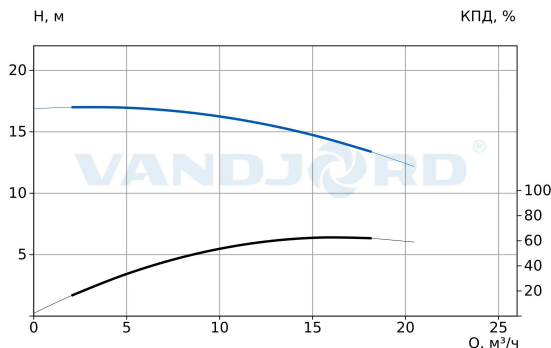
73113103 TPV 40-150-1.1/2 Q-A-B-E
