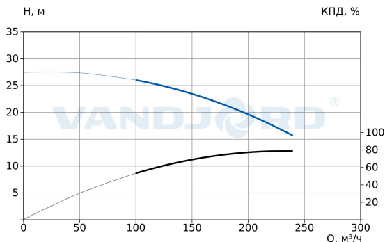
74147002 CRV 200-1CN BI-D-E-HUBE-E
