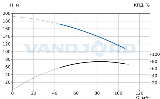
74144019 CRV 90-6CN A-D-E-HQQE-E
