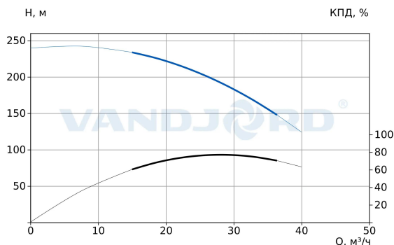
74141054 CRV 32-13CN A-D-E-HQQE-E
