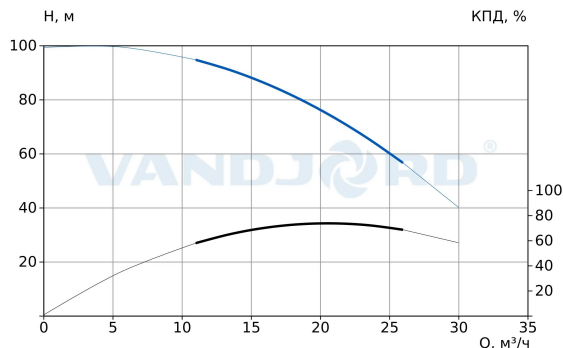
74139019 CRV 20-7CN A-D-E-HQQE-E
