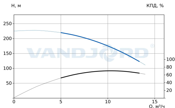
74137032 CRV 10-22CN A-D-E-HQQE-E
