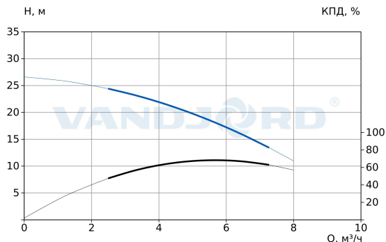
74135026 CRV 5-4CN A-D-E-HQQE-E
