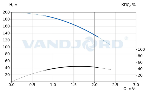
74131043 CRV 1-33CN A-D-E-HQQE-E
