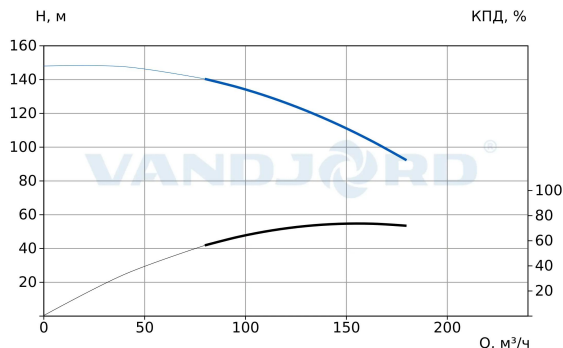
74126717 CRV 150-6-2C A-D-E-HUBE-E
