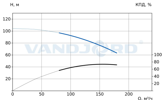
74126710 CRV 150-4-1C A-D-E-HUBE-E
