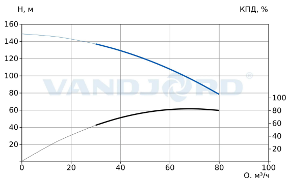
74123725 CRV 64-5C A-D-E-HQQE-E
