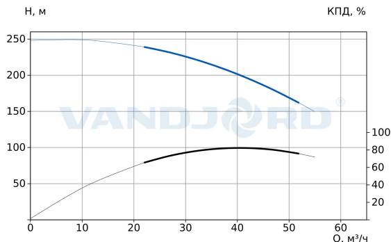
74122732 CRV 45-10-2C A-D-E-HQQE-E
