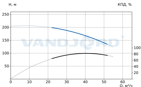
74122729 CRV 45-8C A-D-E-HQQE-E
