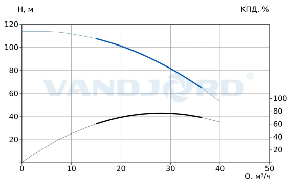
74121736 CRV 32-6C A-D-E-HQQE-E
