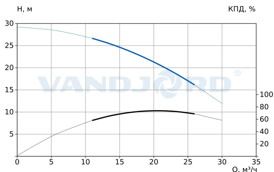
74119710 CRV 20-2C A-D-E-HQQE-E
