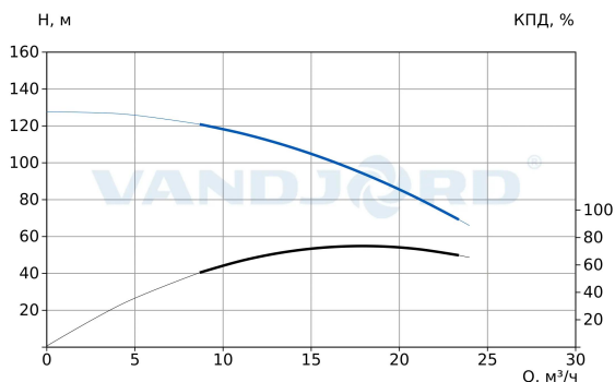
74118724 CRV 15-9C A-D-E-HQQE-E
