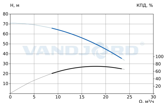
74118720 CRV 15-5C A-D-E-HQQE-E
