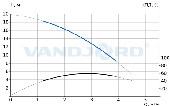
74113745 CRV 3-3C A-D-E-HQQE-E
